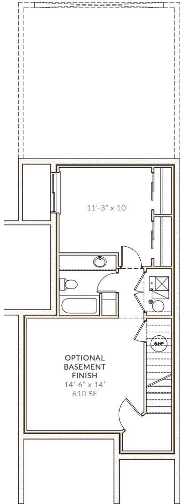
BASEMENT - 639 SF
