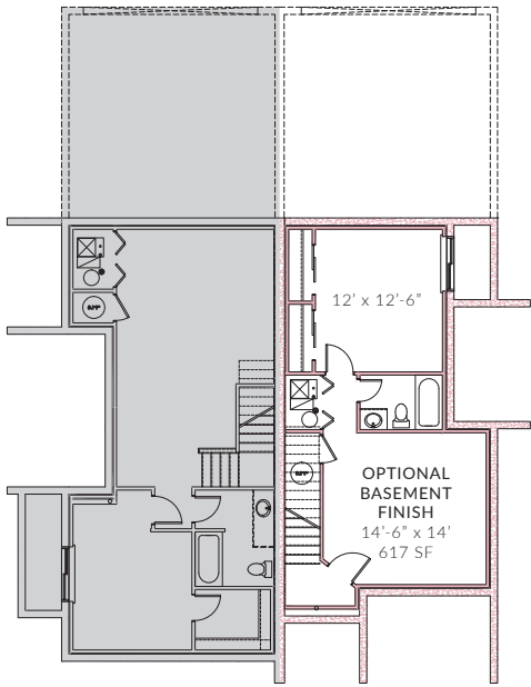
BASEMENT - 639 SF
